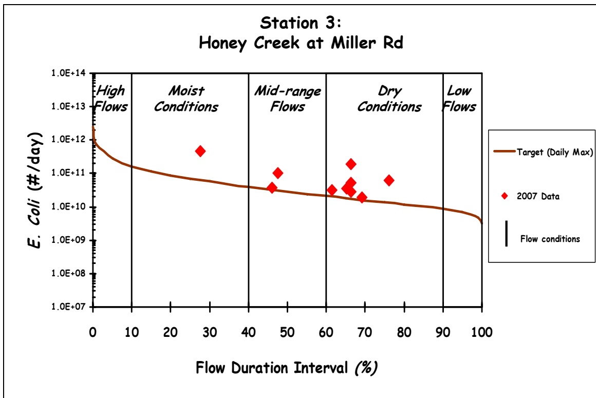
Figure 7. Flow duration curve for Honey Creek at Miller Road (Station 3). Curve is based on E. coli Data and USGS Gage Duration Interval 04173500, and a drainage area of 22.3 square miles.
