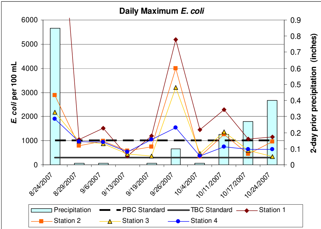
Figure 2. Daily Maximum E. coli sampling results from Honey Creek (Stations 1-4).
