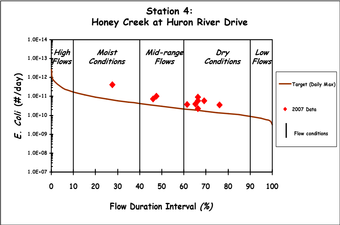
Figure 8. Flow duration curve for Honey Creek at Huron River Drive (Station 4). Curve is based on E. coli Data and USGS Gage Duration Interval 04173500, and a drainage area of 23.3 square miles.
