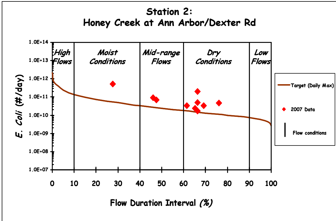
Figure 6. Flow duration curve for Honey Creek at Ann Arbor/Dexter Road (Station 2). Curve is based on E. coli Data and USGS Gage Duration Interval 04173500, and a drainage area of 18.8 square miles.
