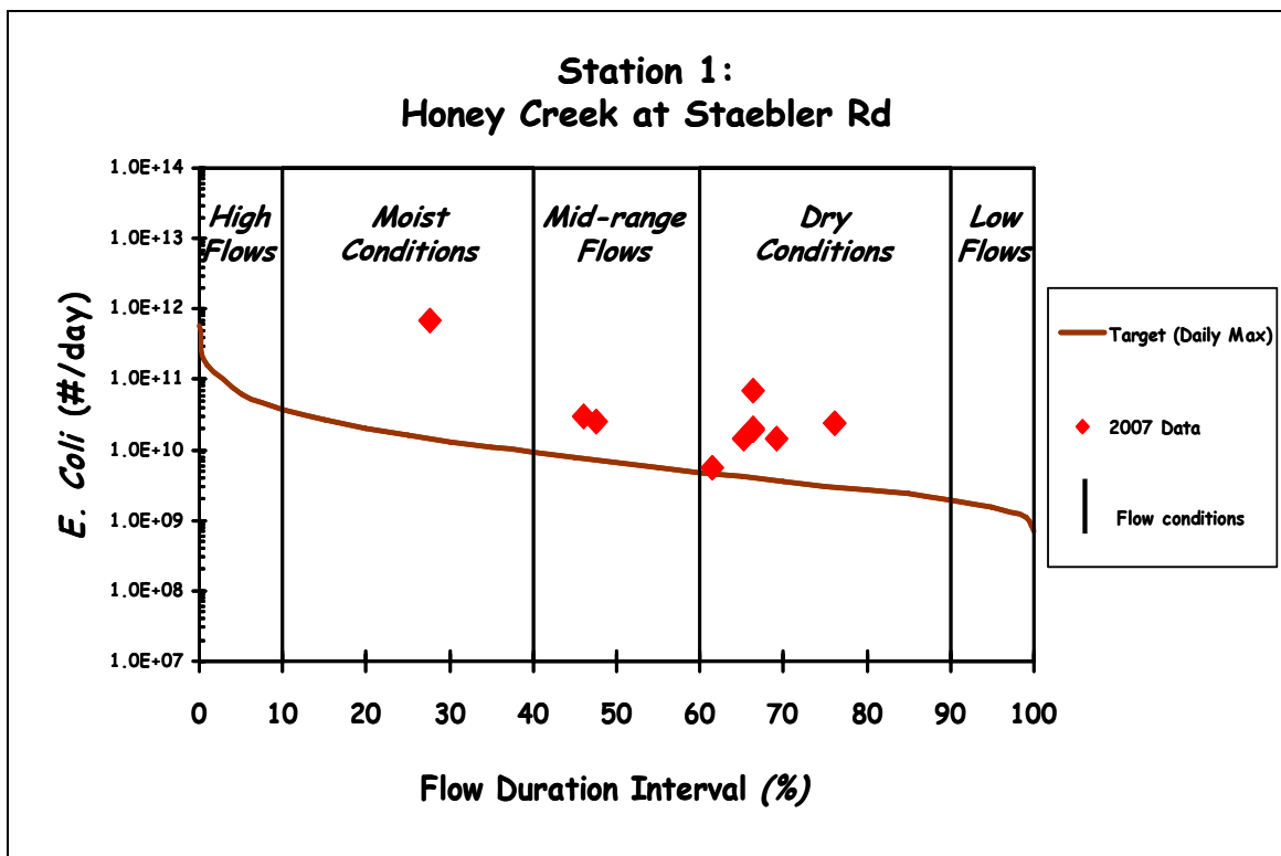
Figure 5. Flow duration curve for Honey Creek at Staebler Road (Station 1). Curve is based on E. coli Data and USGS Gage Duration Interval 04173500, and a drainage area of 5.1 square miles.
