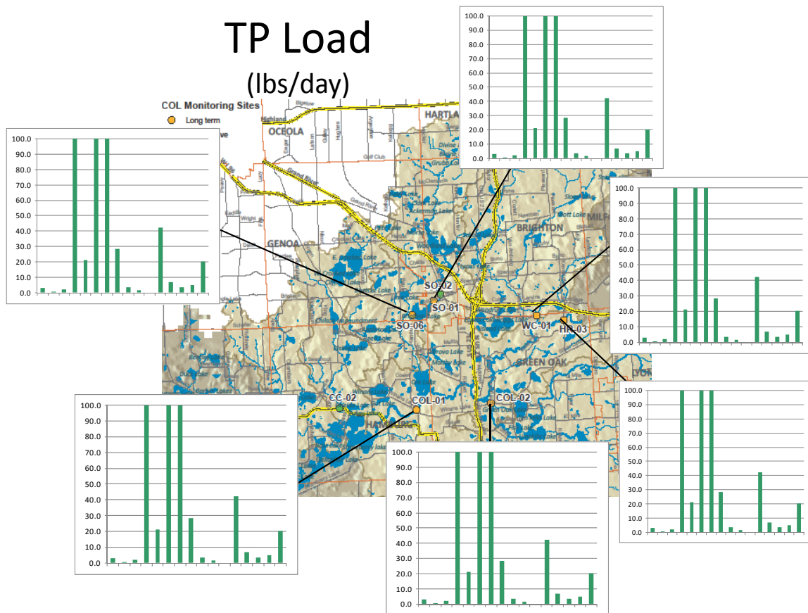
Figure 6. Total Phosphorus loading for monitoring site in the Chain of Lakes Watershed.
