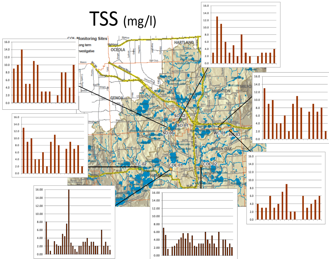
Figure 4. TSS levels at Huron Chain of Lake sites, 2010-2011. Data from 2008-2009 included for Huron River at Hamburg and Davis Creek.
