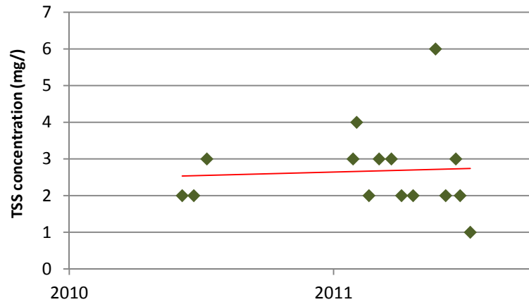
TSS @ Huron River - Hamburg
