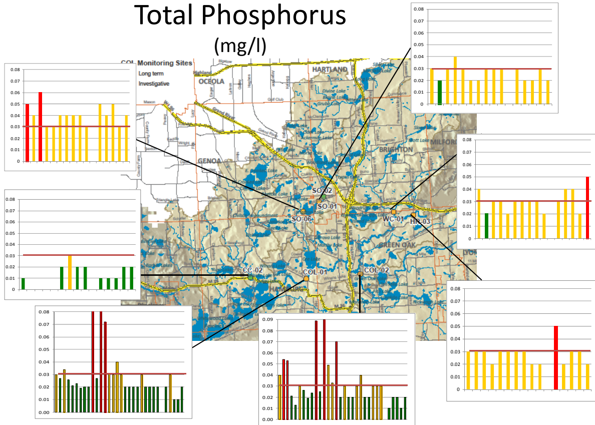
Figure 3. Total Phosphorus concentrations over time at sites in the Huron Chain of Lakes Watershed. The TMDL target level of 0.03 mg/l is indicated. Values in yellow match or exceed this threshold and values in red exceed 0.05 mg/l.
